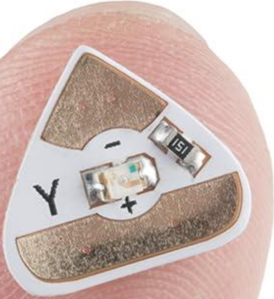
Chibitronic LED
